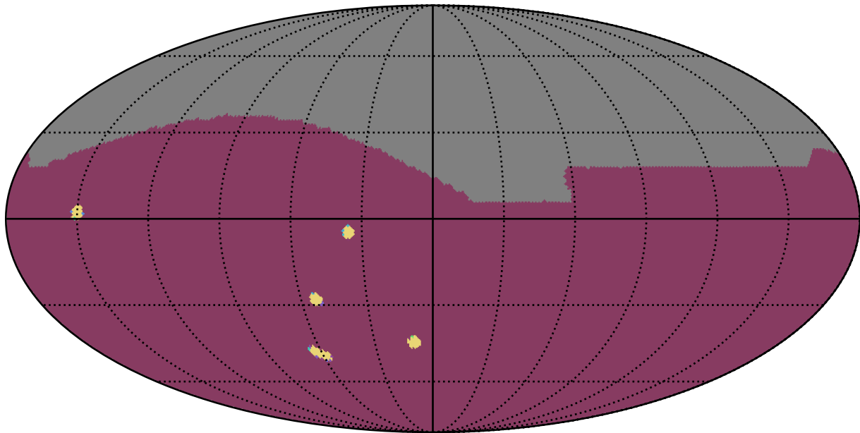
too_ignore_100_4v3.4_10yrs All sky: NumberOfQuickRevisits
