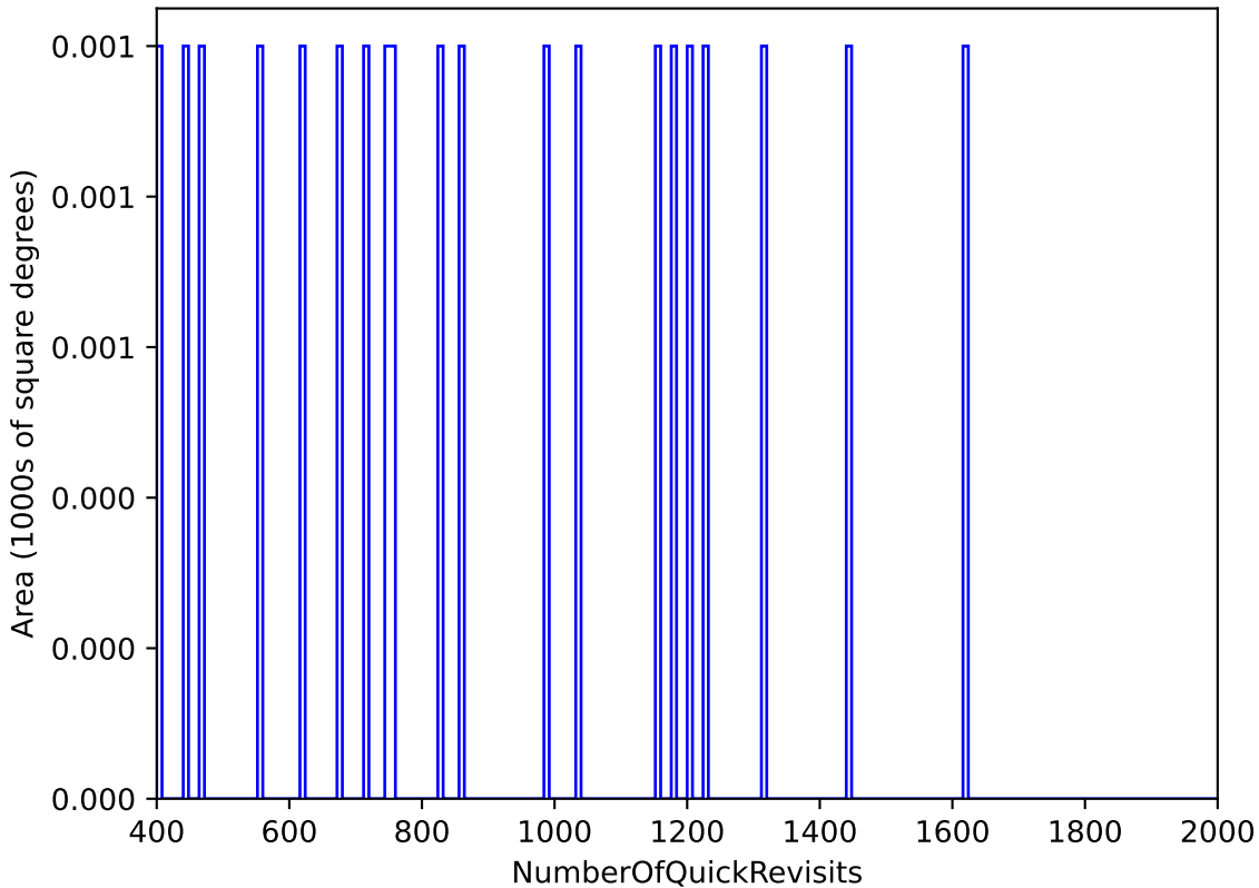
too_ignore_100_4v3.4_10yrs All sky: NumberOfQuickRevisits
