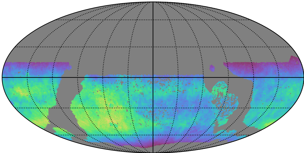
too_ignore_100_4v3.4_10yrs WFD z band: Normalized Teff
