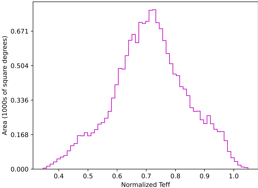
too_ignore_100_4v3.4_10yrs WFD z band: Normalized Teff
