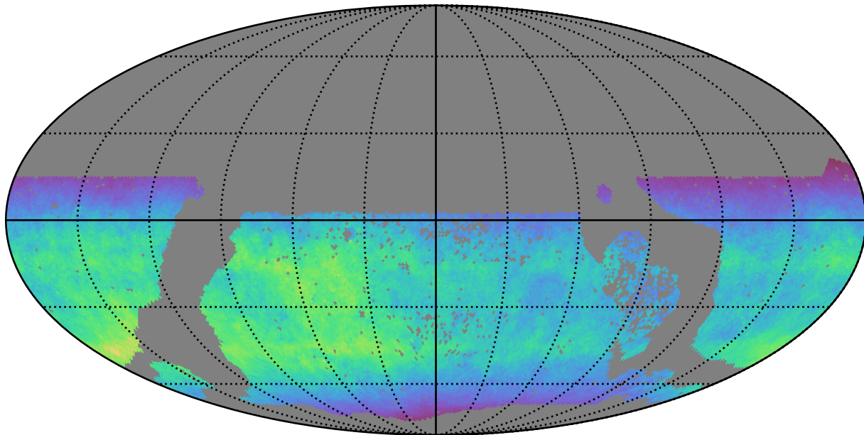
too_ignore_100_4v3.4_10yrs WFD y band: Normalized Teff
