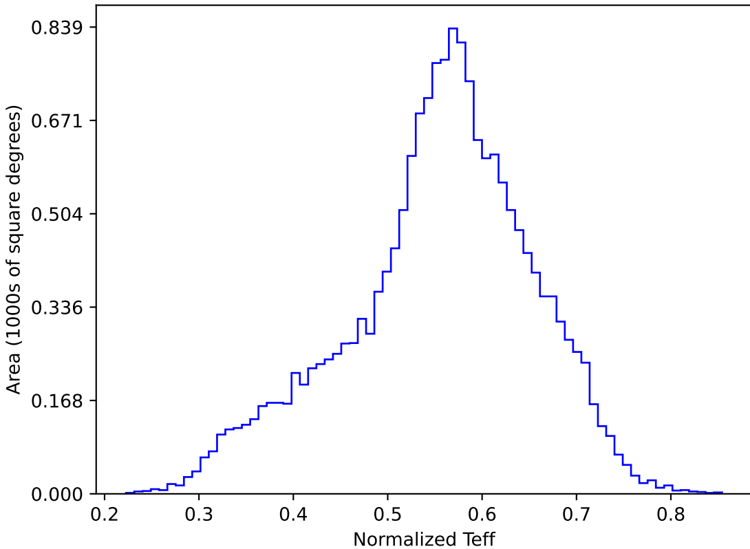
too_ignore_100_4v3.4_10yrs WFD y band: Normalized Teff
