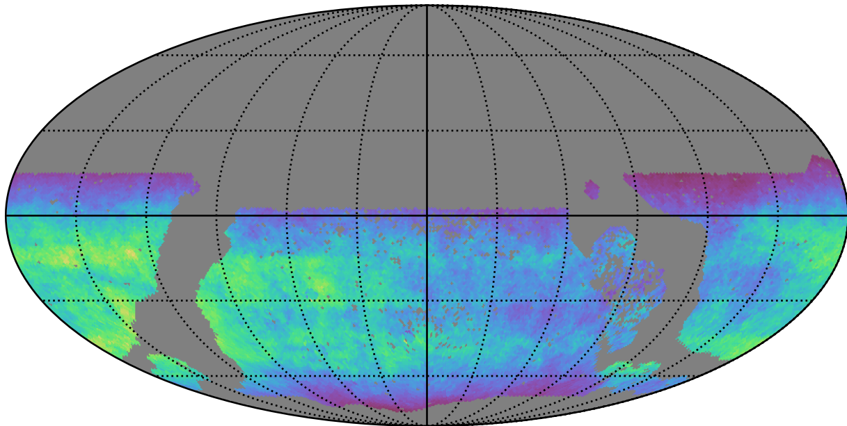
too_ignore_100_4v3.4_10yrs WFD u band: Normalized Teff
