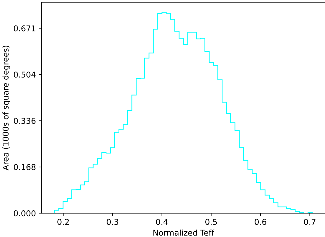
too_ignore_100_4v3.4_10yrs WFD u band: Normalized Teff
