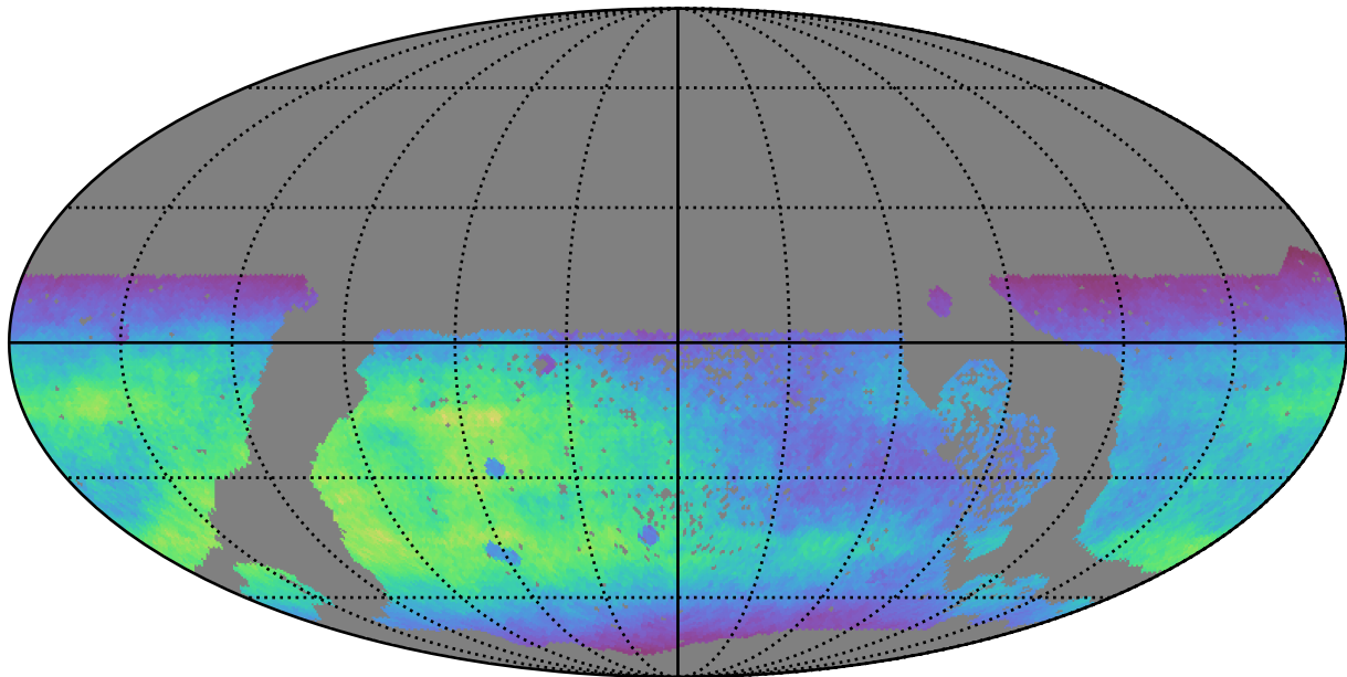
too_ignore_100_4v3.4_10yrs WFD r band: Normalized Teff
