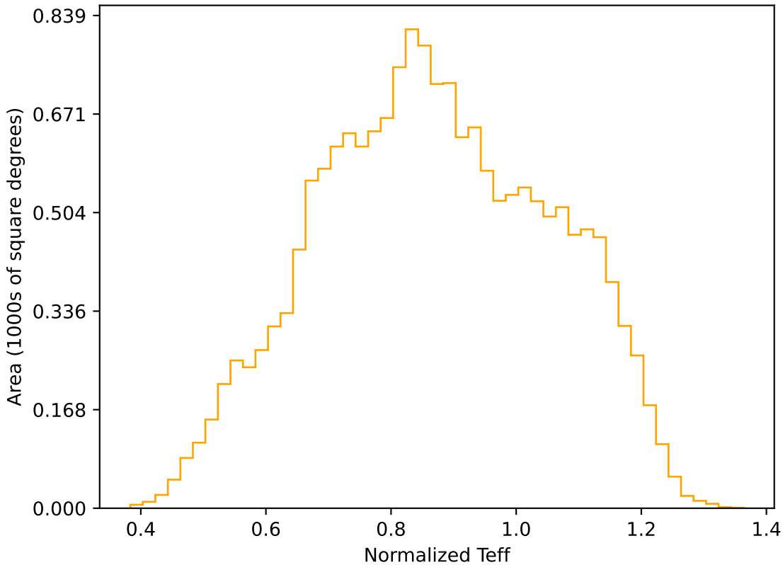
too_ignore_100_4v3.4_10yrs WFD r band: Normalized Teff
