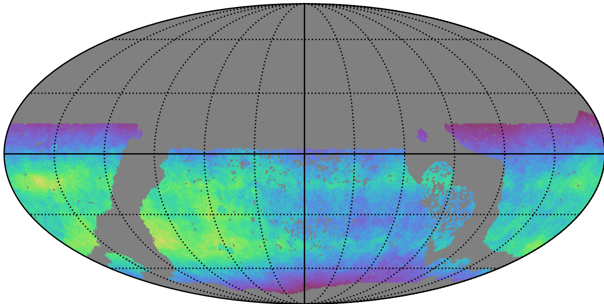
too_ignore_100_4v3.4_10yrs WFD i band: Normalized Teff
