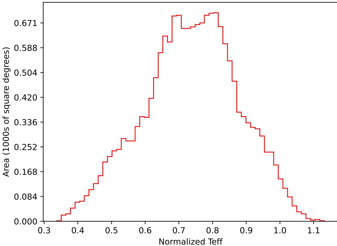
too_ignore_100_4v3.4_10yrs WFD i band: Normalized Teff
