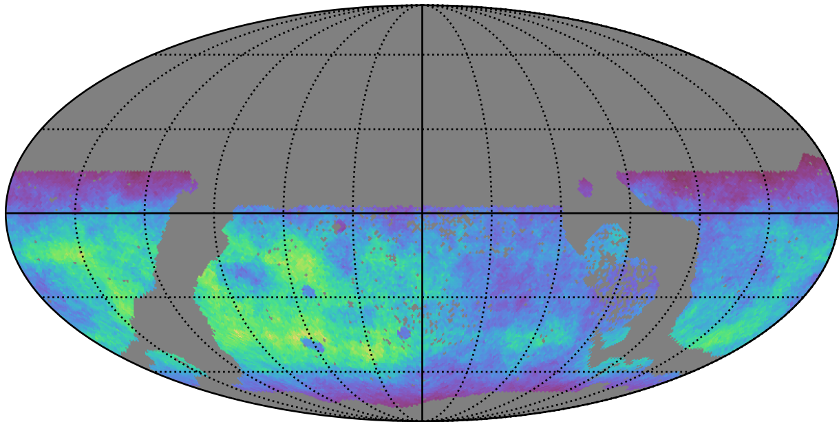
too_ignore_100_4v3.4_10yrs WFD g band: Normalized Teff
