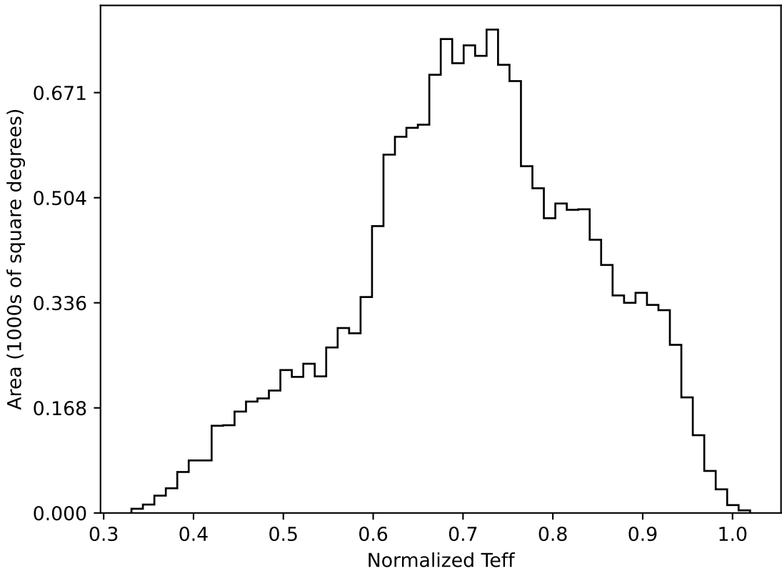
too_ignore_100_4v3.4_10yrs WFD all bands: Normalized Teff
