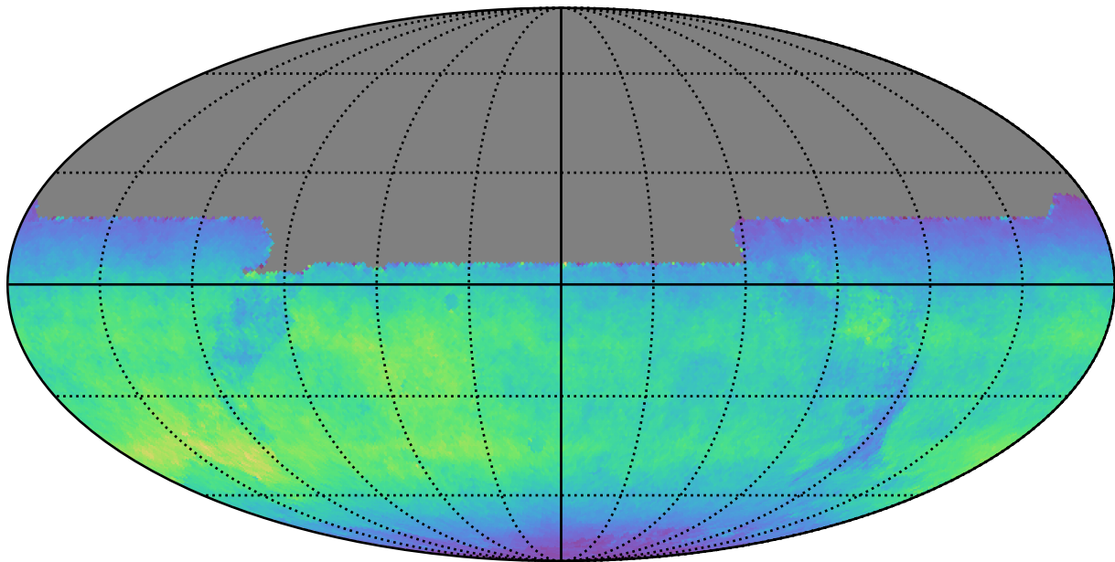
too_ignore_100_4v3.4_10yrs All sky y band: Normalized Teff
