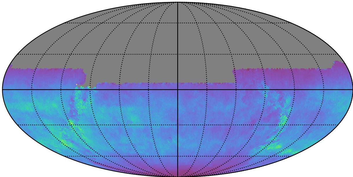
too_ignore_100_4v3.4_10yrs All sky u band: Normalized Teff
