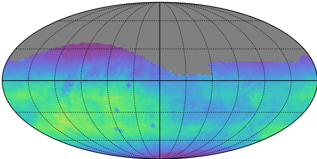
too_ignore_100_4v3.4_10yrs All sky r band: Normalized Teff
