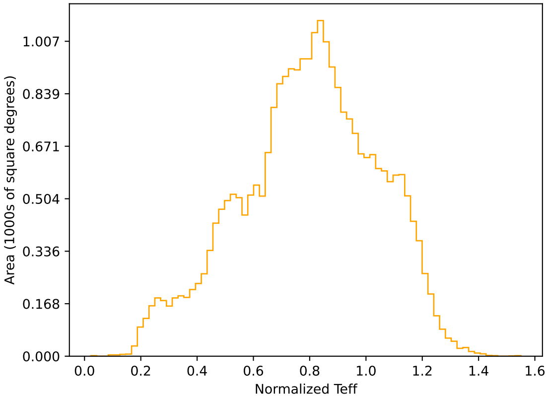
too_ignore_100_4v3.4_10yrs All sky r band: Normalized Teff
