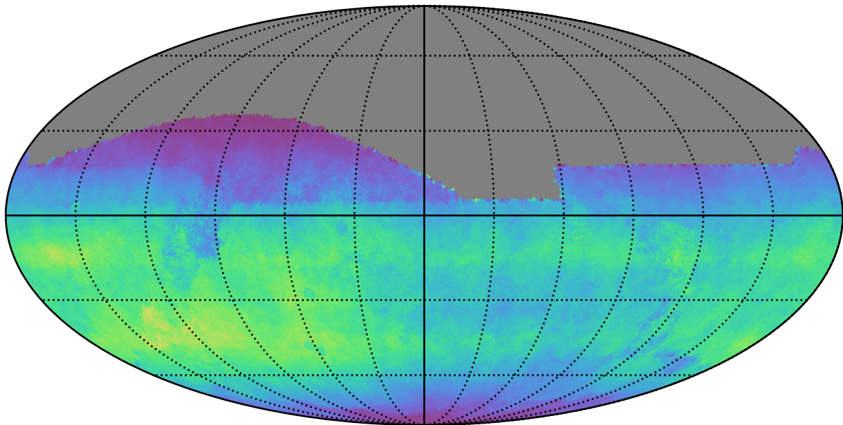
too_ignore_100_4v3.4_10yrs All sky i band: Normalized Teff
