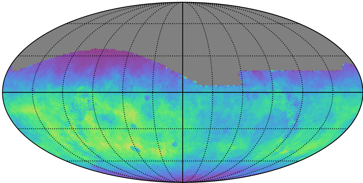
too_ignore_100_4v3.4_10yrs All sky g band: Normalized Teff
