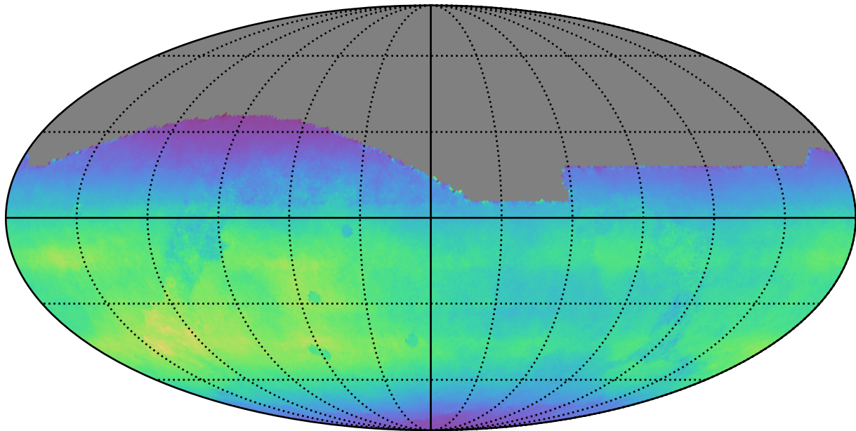
too_ignore_100_4v3.4_10yrs All sky all bands: Normalized Teff
