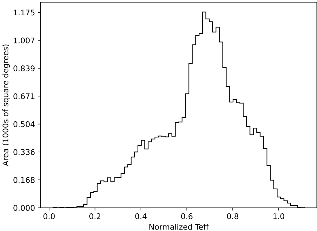
too_ignore_100_4v3.4_10yrs All sky all bands: Normalized Teff
