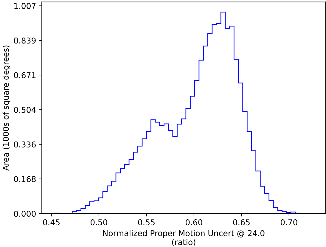
too_ignore_100_4v3.4_10yrs WFD: Normalized Proper Motion Uncert @ 24.0
