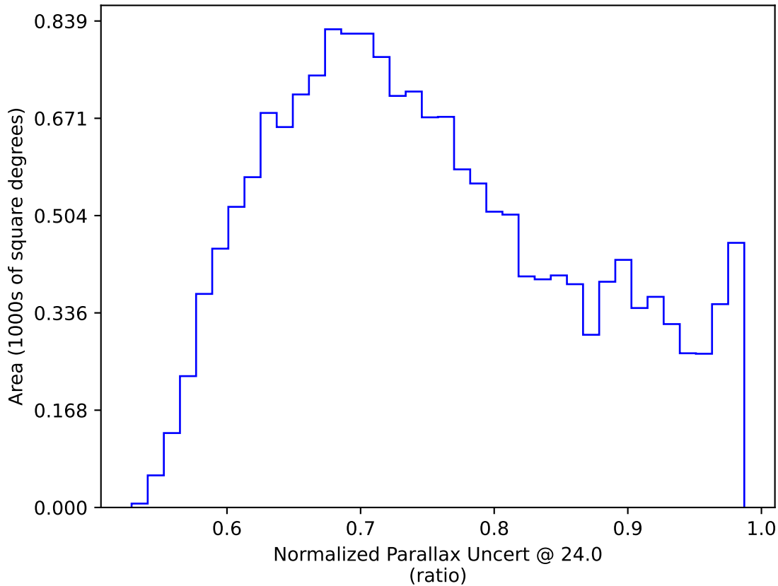
too_ignore_100_4v3.4_10yrs WFD: Normalized Parallax Uncert @ 24.0
