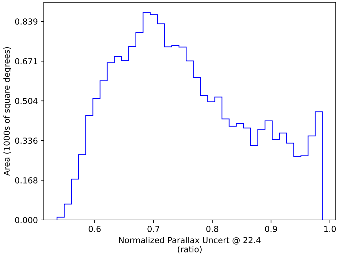
too_ignore_100_4v3.4_10yrs WFD: Normalized Parallax Uncert @ 22.4
