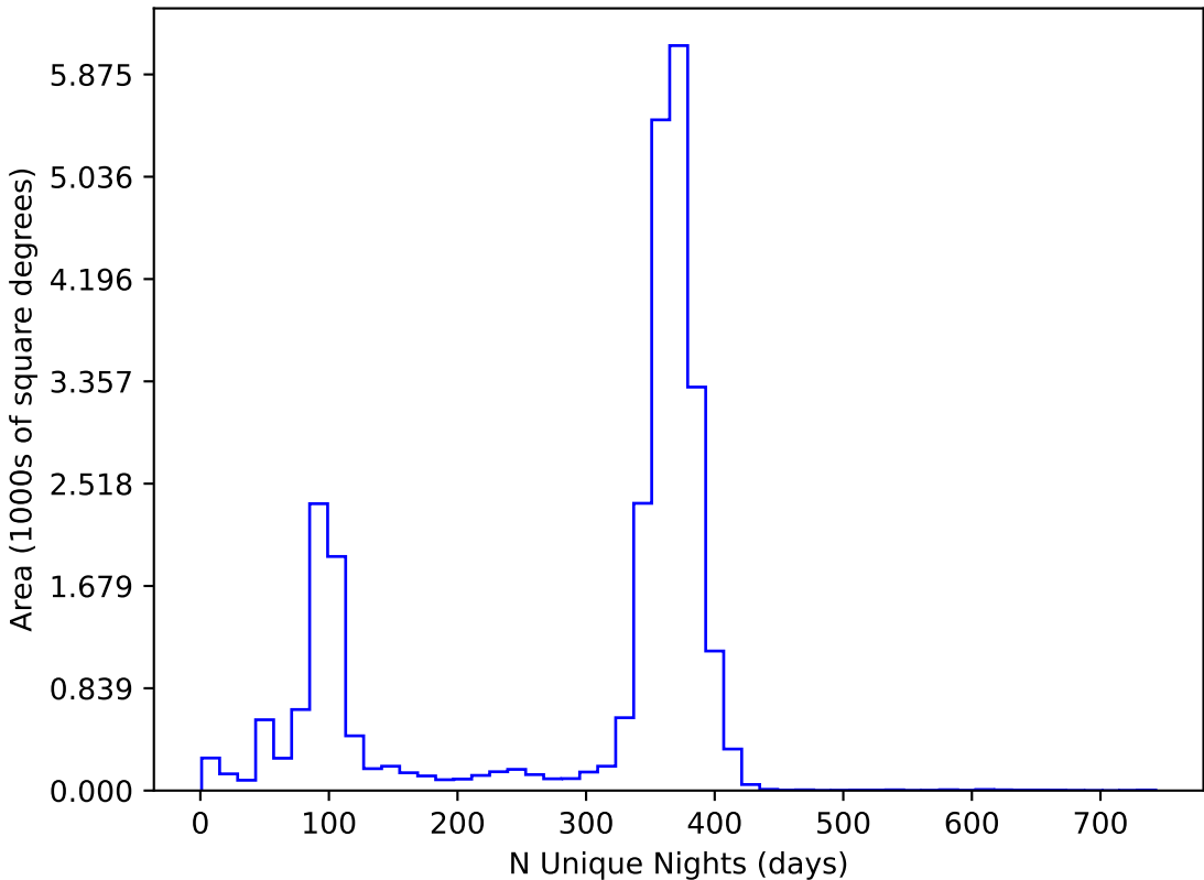
too_ignore_100_4v3.4_10yrs All sky all bands: N Unique Nights
