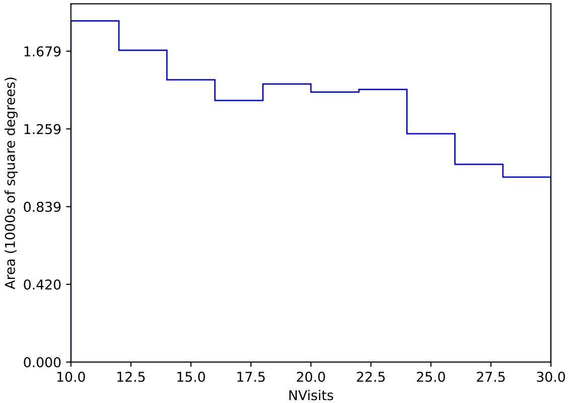
too_ignore_100_4v3.4_10yrs Yr 3-4 y band: NVisits
