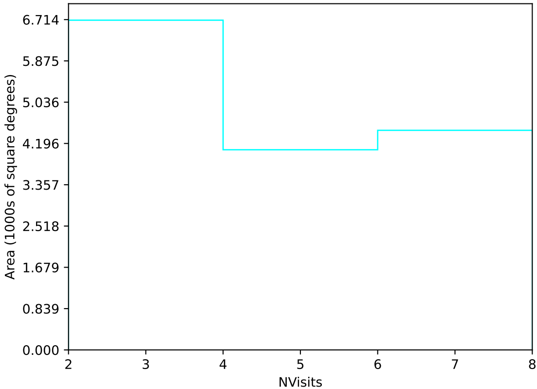
too_ignore_100_4v3.4_10yrs Yr 3-4 u band: NVisits
