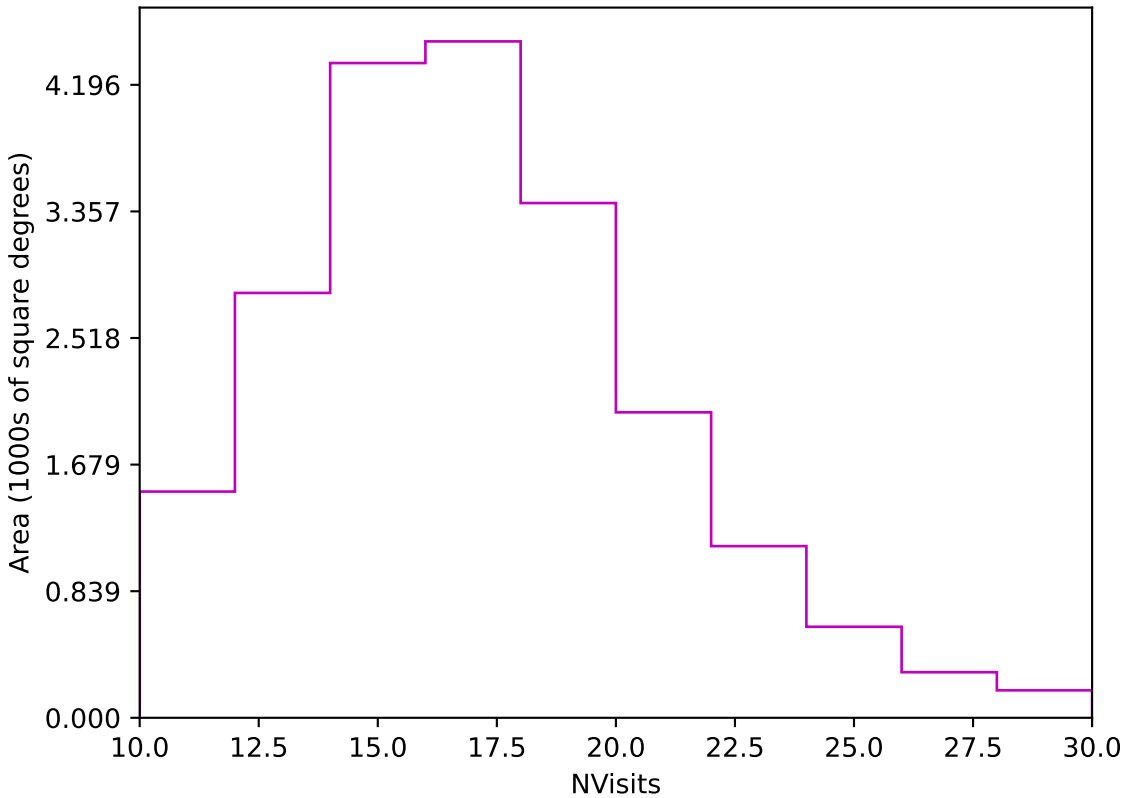
too_ignore_100_4v3.4_10yrs Yr 1 z band: NVisits
