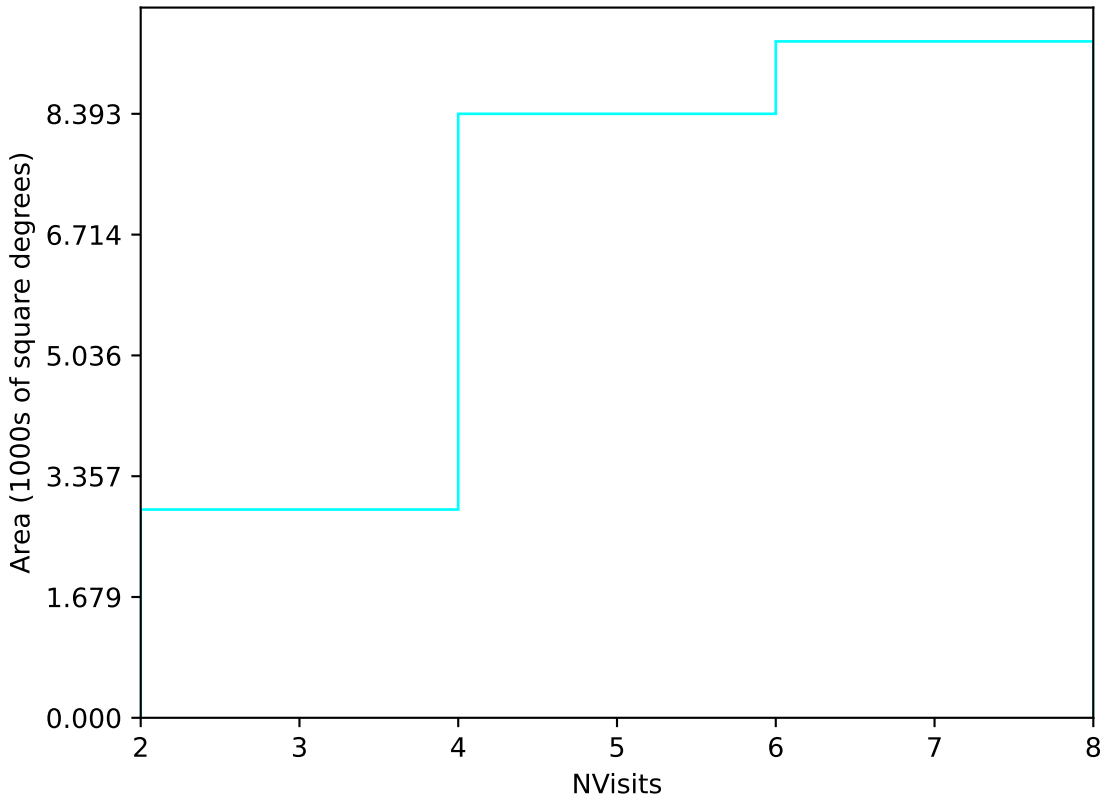
too_ignore_100_4v3.4_10yrs Yr 1 u band: NVisits
