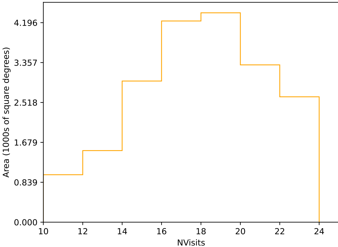
too_ignore_100_4v3.4_10yrs Yr 1 r band: NVisits
