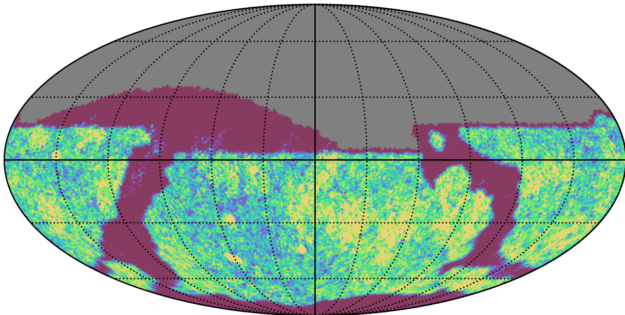
too_ignore_100_4v3.4_10yrs Yr 1 i band: NVisits
