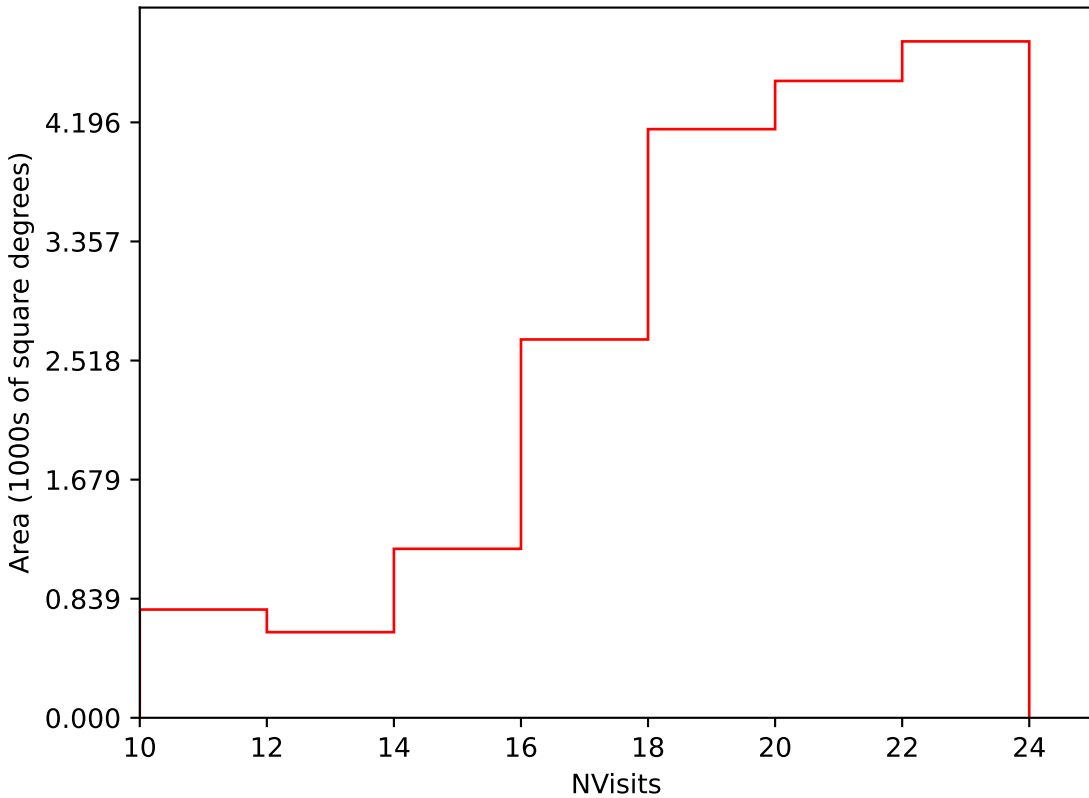
too_ignore_100_4v3.4_10yrs Yr 1 i band: NVisits
