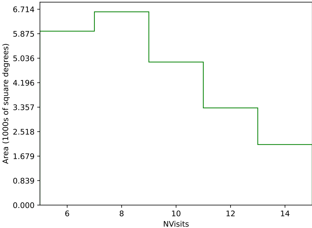
too_ignore_100_4v3.4_10yrs Yr 1 g band: NVisits
