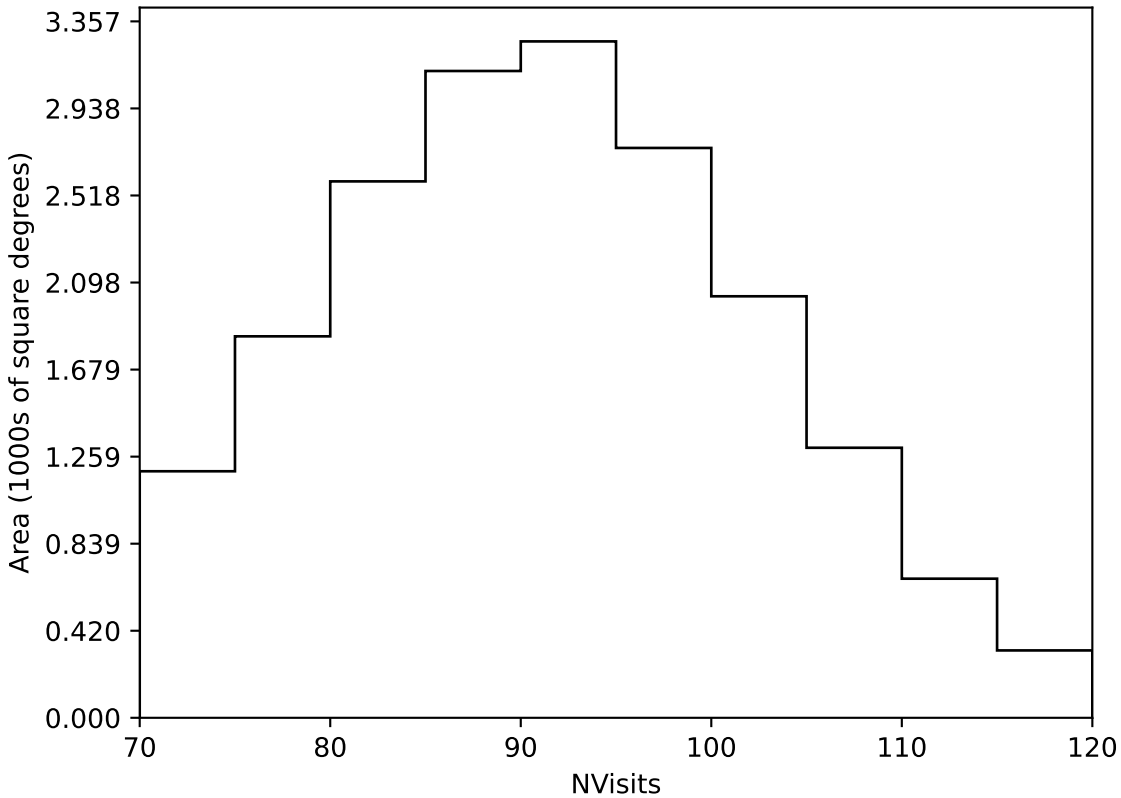
too_ignore_100_4v3.4_10yrs Yr 1 all bands: NVisits
