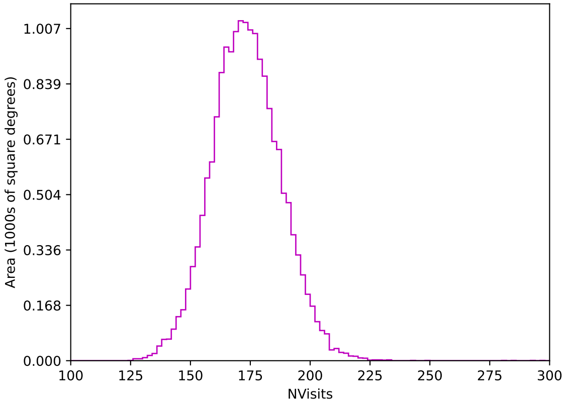
too_ignore_100_4v3.4_10yrs WFD z band: NVisits
