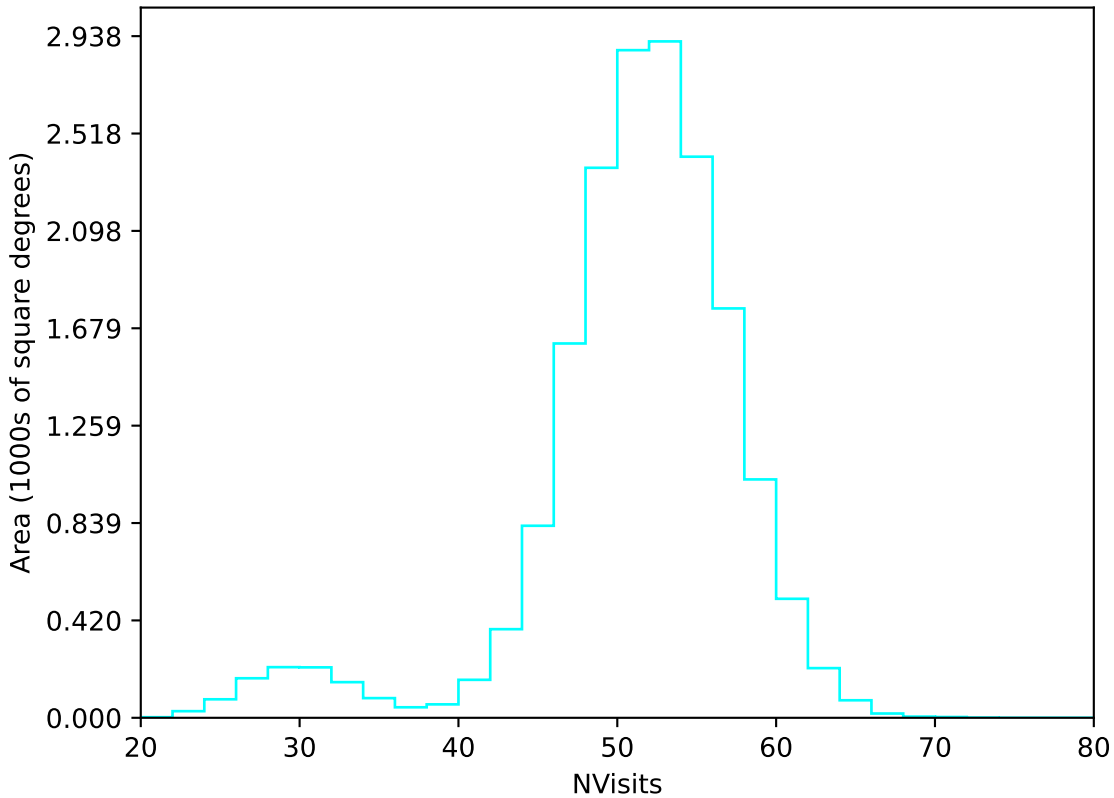
too_ignore_100_4v3.4_10yrs WFD u band: NVisits
