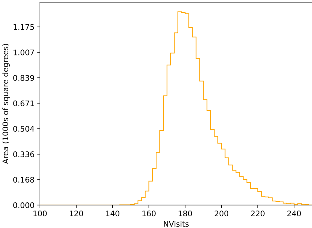
too_ignore_100_4v3.4_10yrs WFD r band: NVisits
