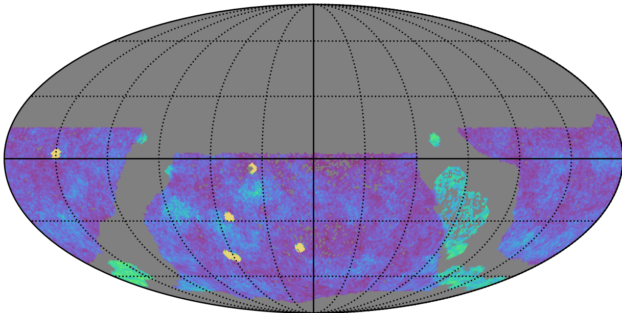
too_ignore_100_4v3.4_10yrs WFD g band: NVisits
