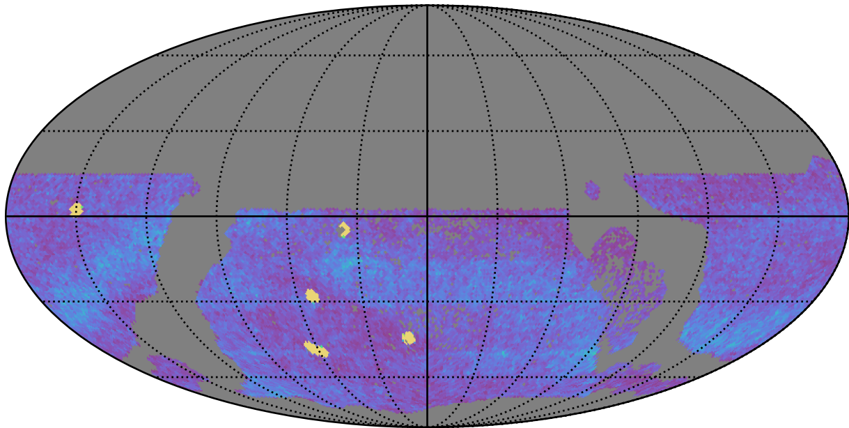
too_ignore_100_4v3.4_10yrs WFD all bands: NVisits
