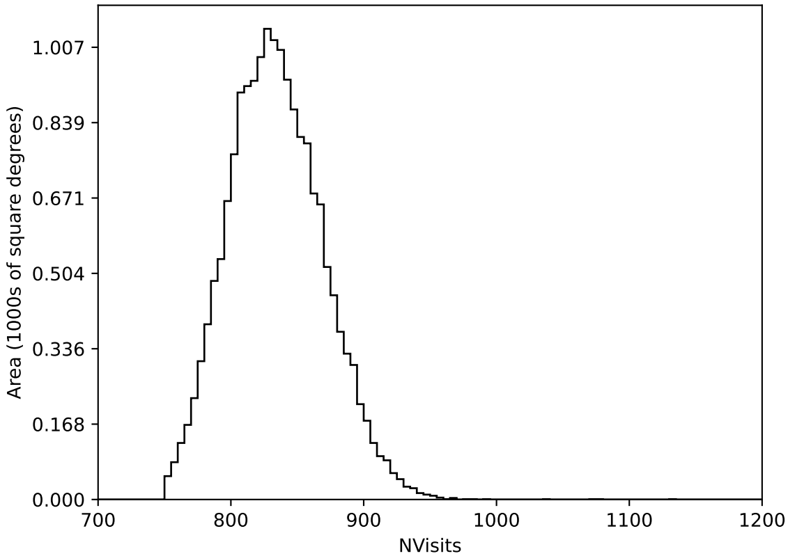
too_ignore_100_4v3.4_10yrs WFD all bands: NVisits
