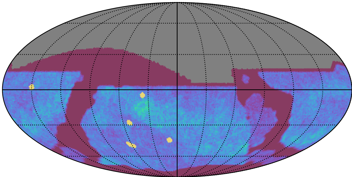
too_ignore_100_4v3.4_10yrs All sky z band: NVisits
