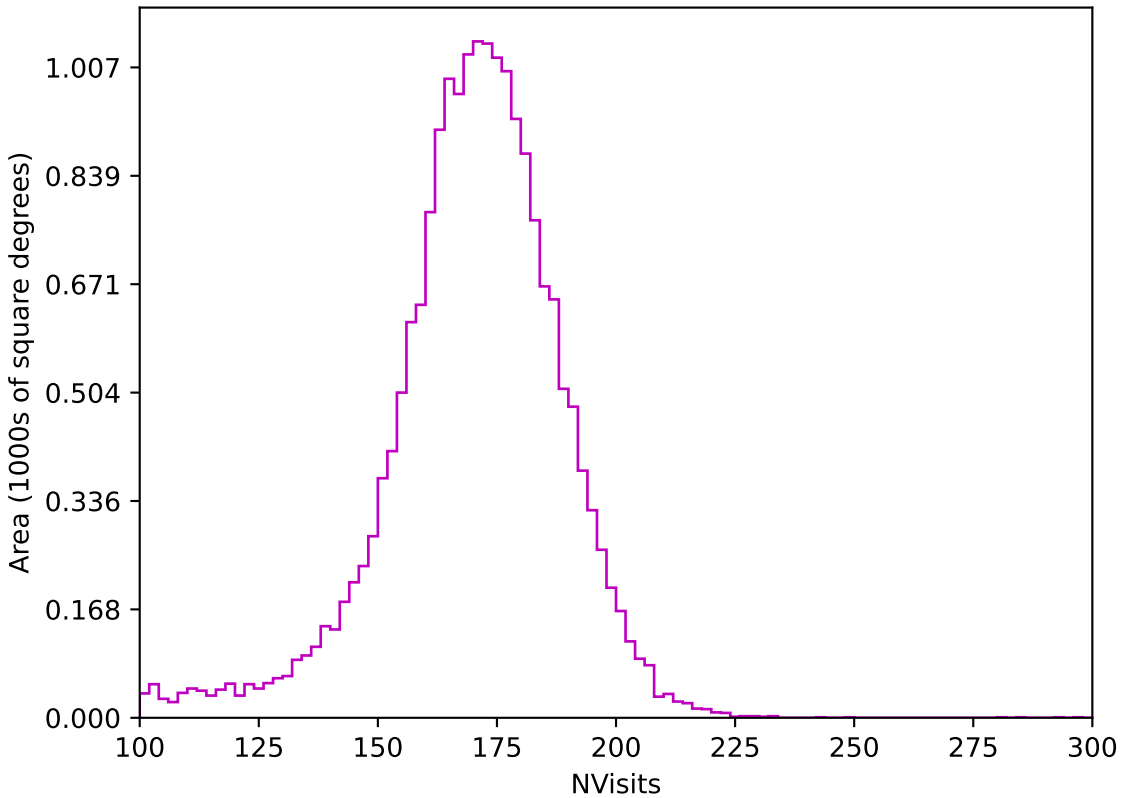
too_ignore_100_4v3.4_10yrs All sky z band: NVisits
