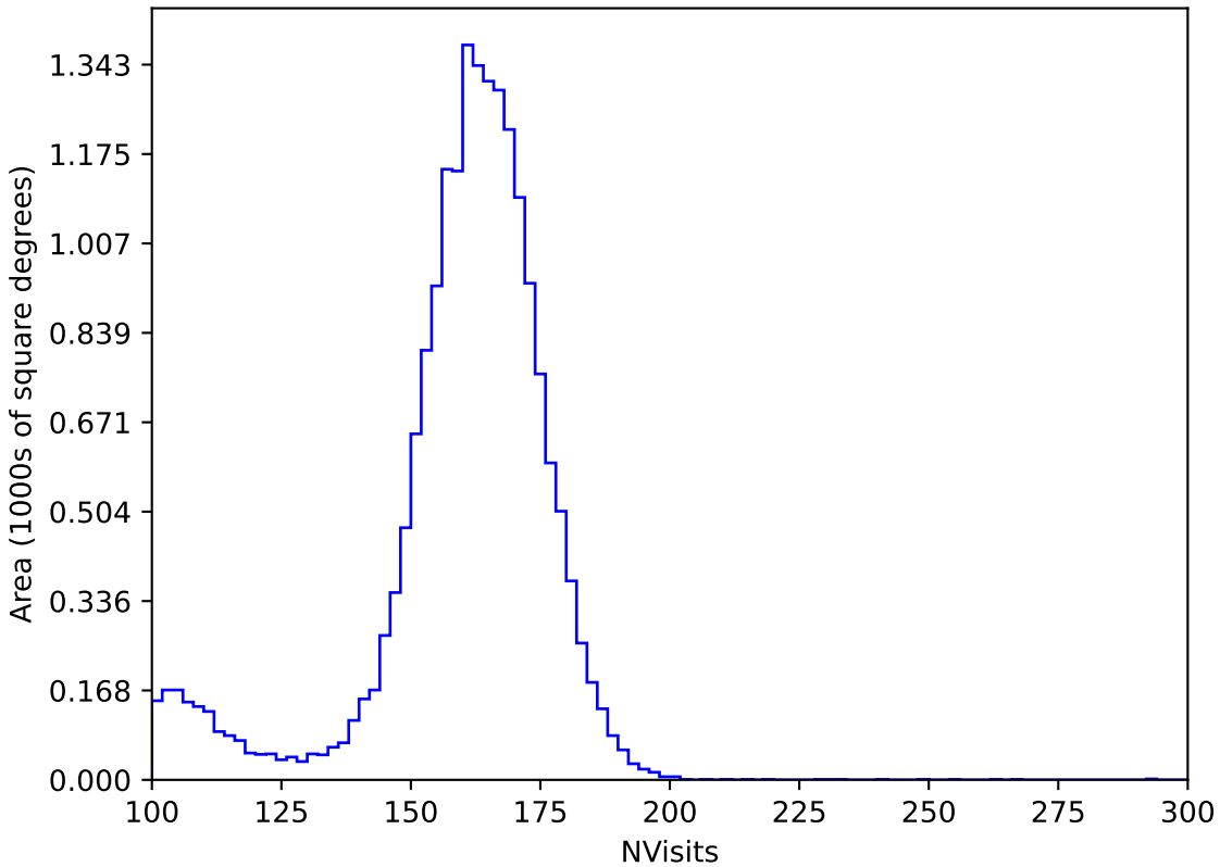
too_ignore_100_4v3.4_10yrs All sky y band: NVisits
