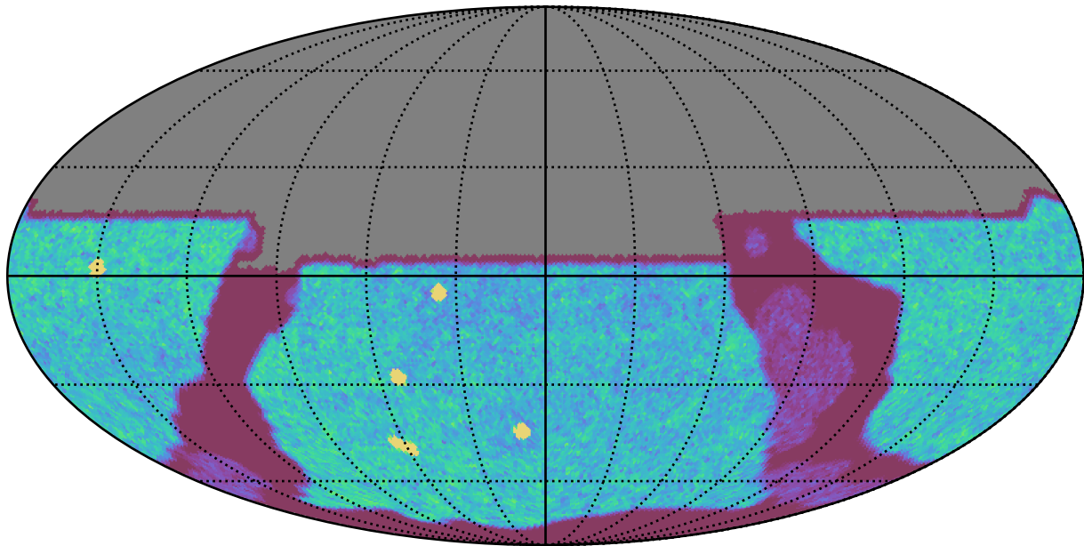
too_ignore_100_4v3.4_10yrs All sky u band: NVisits
