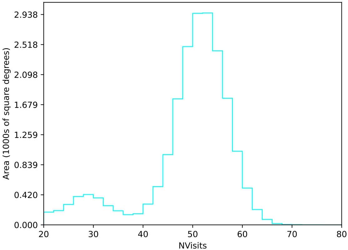
too_ignore_100_4v3.4_10yrs All sky u band: NVisits
