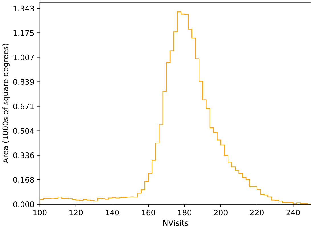
too_ignore_100_4v3.4_10yrs All sky r band: NVisits
