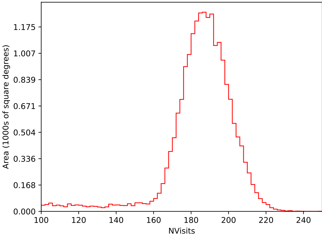
too_ignore_100_4v3.4_10yrs All sky i band: NVisits
