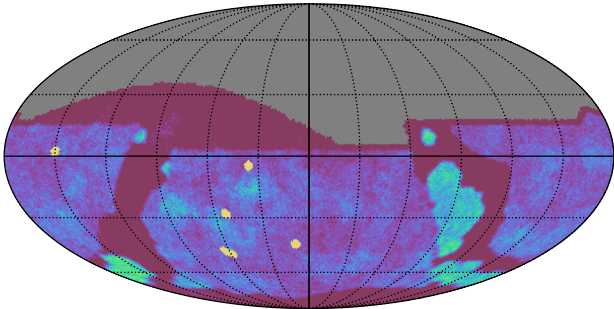
too_ignore_100_4v3.4_10yrs All sky g band: NVisits
