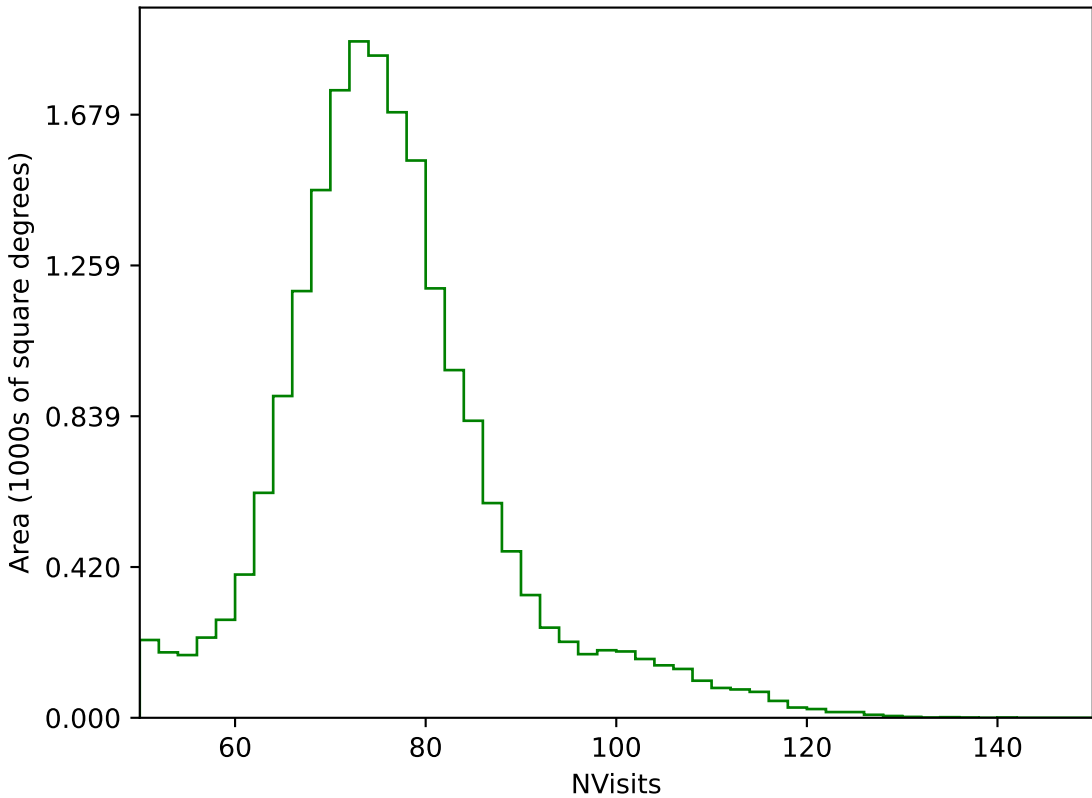
too_ignore_100_4v3.4_10yrs All sky g band: NVisits
